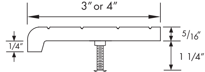
CAST-ON ANCHOR
