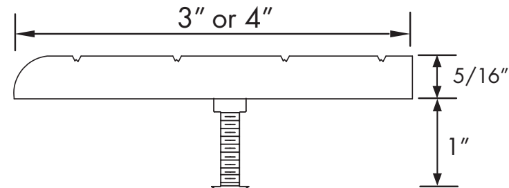
CAST-ON ANCHOR
