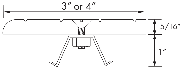
WING ANCHOR
