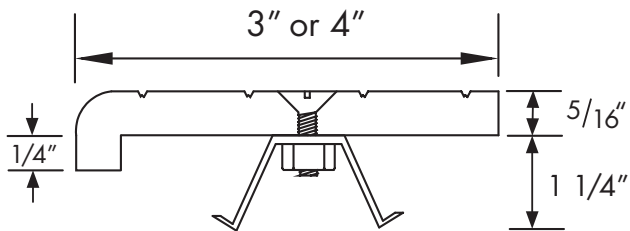
WING ANCHOR
