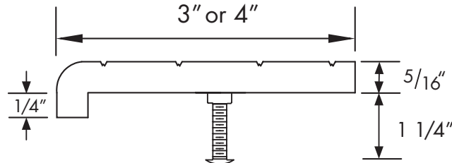
CAST-ON ANCHOR
